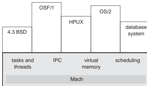
Figure B.1 Mach 3 structure.
